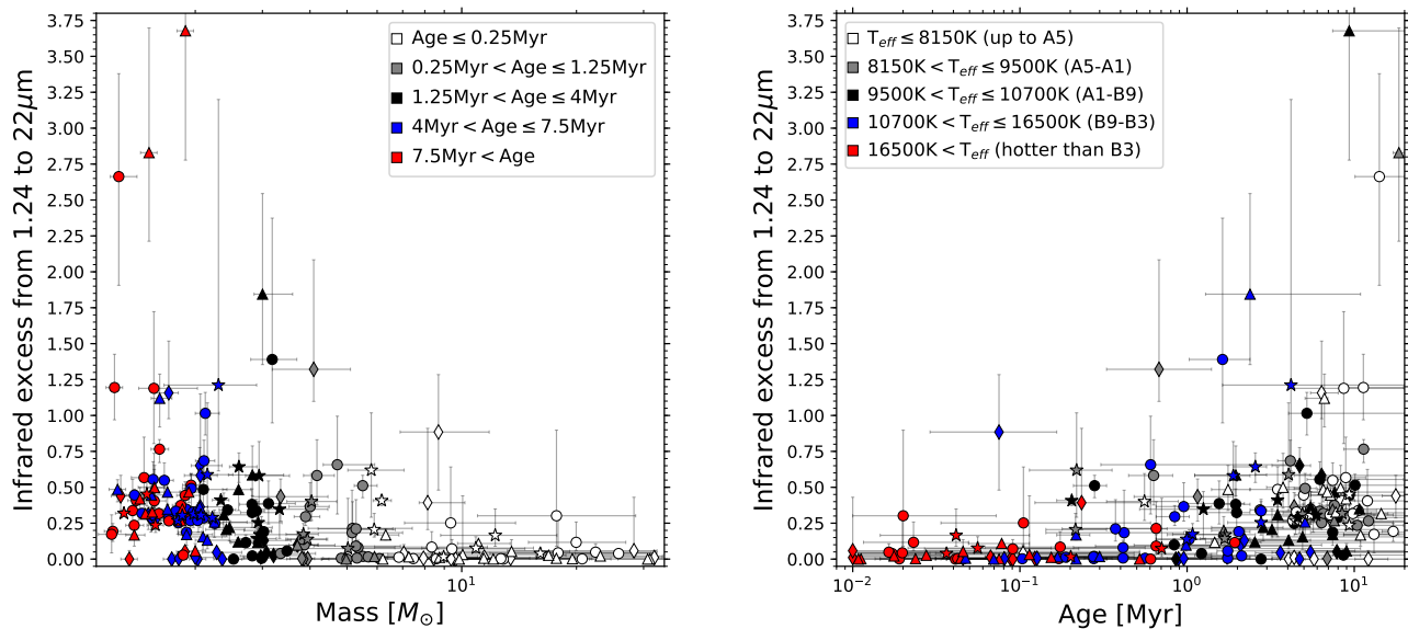
Fig. 4. Left: IR excess in the range 1.24 – 22 \mu m vs. estimated mass of the objects. The most massive objects (more massive than \sim 7M_{\odot} ) barely show an IR excess. Right: IR excess in the range 1.24 – 22 \mu m vs. estimated age. Ages and effective temperatures are respectively colour coded in the legend. The symbols stand for the H \alpha line profiles: circles (double-peaked), triangles (single-peaked), stars (P-Cygni profile) and diamonds (no information). We note that although it is not necessarily a one-to-one correlation, lower ages correspond to higher masses.
