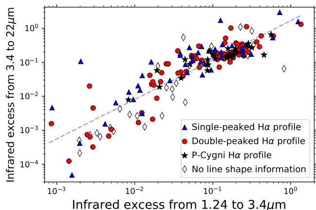
Fig. 5. IR excess in the range 3.4 – 22 \mu\text{m} (MIR excess) vs. IR excess in the range 1.24 – 3.4 \mu\text{m} (NIR excess). The symbols stand for the H\alpha line profiles: circles (double-peaked), triangles (single-peaked), stars (P-Cygni profile) and diamonds (no information). A linear fit in the log space is shown in blue ( \log(\text{Mid IR}_{\text{excess}}) = 1.16 \log(\text{Near IR}_{\text{excess}}) + 0.23 , r = 0.88 ).
