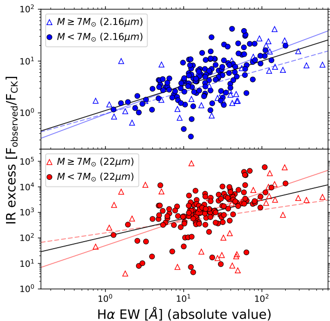
Fig. 7. 2.16\mu\text{m} (blue markers) and 22\mu\text{m} (red markers) IR excesses defined as F_{\text{observed}}/F_{\text{CK}} vs. H\alpha EW (absolute value). We note that this IR excess indicator is a flux ratio and not the one described in Eq. 2 where we integrated under the SED. Dots are Herbig Ae/Be stars with M < 7M_{\odot} and triangles are Herbig Ae/Be stars with M > 7M_{\odot} . Lines are linear fits to the data, dashed for HAeBes with M > 7M_{\odot} and in solid colours for HAeBes with M < 7M_{\odot} ; black solid lines are the linear fits for all the sources (equations and correlation coefficients for these fits to all the sources for all the IR bands can be seen in Table 3). We highlight the difference in the scale of the vertical axis between the two panels.
